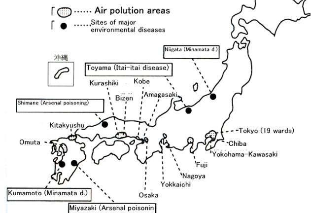
Sites of air pollution and major environmental diseases
